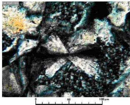
Very fine "bow tie" aggregates of andalusite in matrix of boehmite
